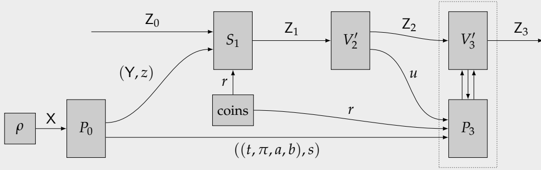
Figure 4: The interaction corresponding to the execution of the coin flipping protocol has been replaced by a simulator S_1 along with a true random string generator (labeled coins ).
