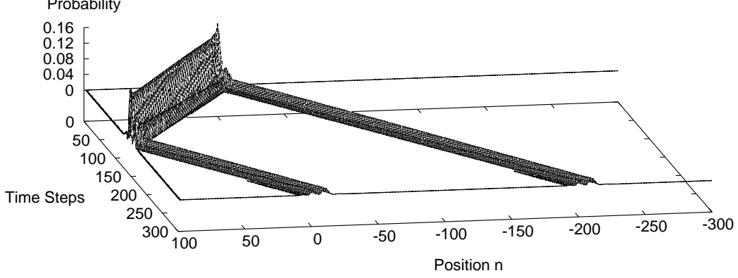
Figure 2: Probability |L(n,t)|^2 + |R(n,t)|^2 as a function of n and t of a Hadamard walk in one-dimension with one absorbing wall started from the initial condition L(n,0) = 0 and R(n,0) \propto \exp(-n^2/100) \cos(\pi n/10) , which is overwhelmingly composed of values of k very close to \pi/10 . Two wavepackets propagate with group velocities \pm v \approx 0.689 (Eq. 33; both +v and -v are seen because the two bands propagate in opposite directions for a given k ); one reflects from the absorbing boundary at position n = 100 with reflection probability P_r \approx 0.184 (Eq. 40).
